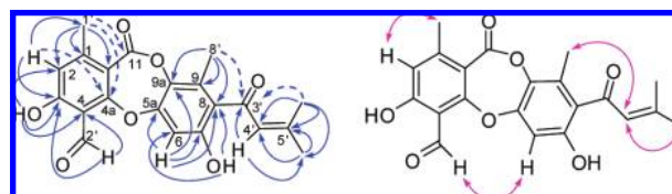
Figure 1. Key HMBC ^2J and ^3J correlations (H \rightarrow C) and ^4J correlations (H \rightarrow C, dashed arrows) and NOESY correlations of mollicellin K ( 1 ).
